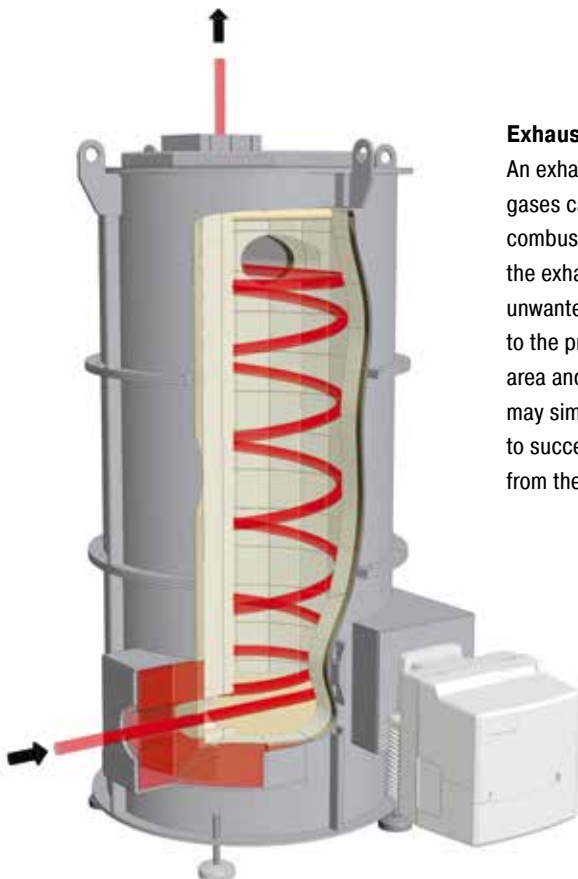
Scheme of a thermal post combustion
